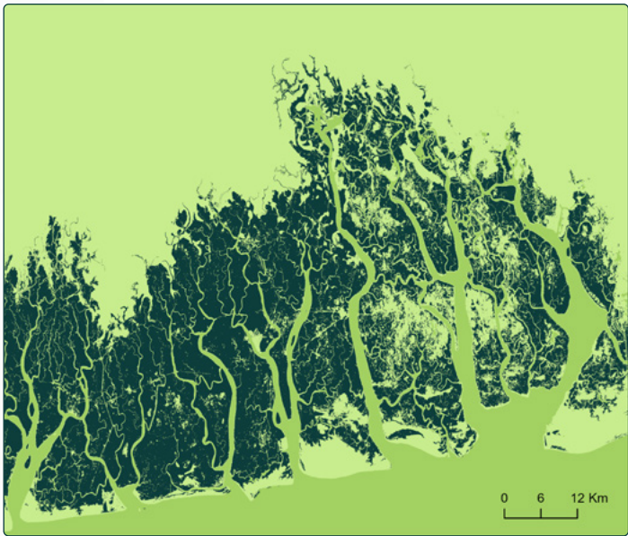
Figure 3. Mangroves in Rivers State, Nigeria. The more open coverage in the eastern half is linked to compounded oil spills over many years 3 .
