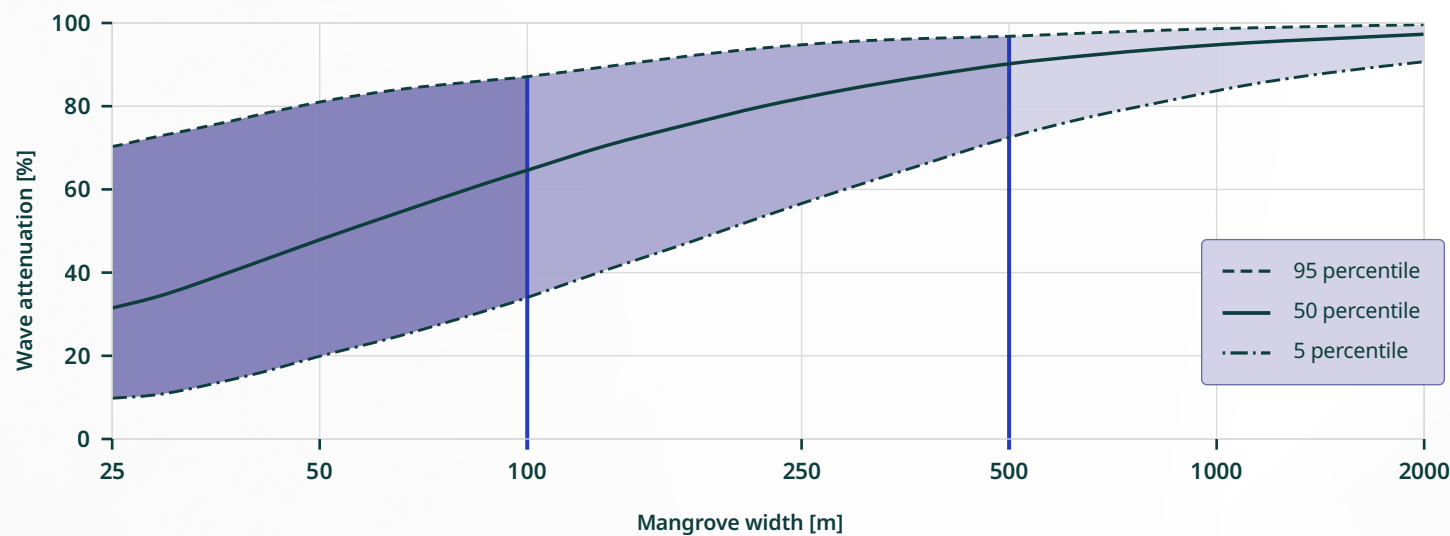
Figure 19: Wave attenuation percentage versus green belt width
