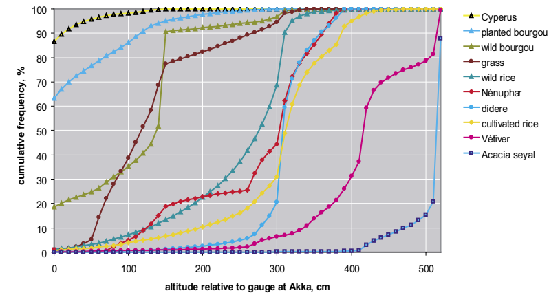
Fig. 6.2 Cumulative frequency distribution (%) of nine vegetation types as a function of the elevation. Bourgou planted by local people has been separated from wild bourgou. Elevation is defined relative to the water-level gauge of Akka. The maximal water level during the last years amounted to 470 cm, on average. Thus, cultivated rice (average altitude 320 cm) is covered by 150 cm at a maximum, wild rice (average elevation 270 cm) by 200 cm and wild bourgou (average altitude 140 cm) by 330 cm.
