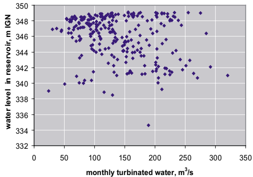
Fig. II.1. Sélingué: turbine flow versus reservoir level
