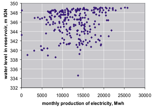
Fig. II.3. Sélingué: reservoir level versus monthly generated energy.
