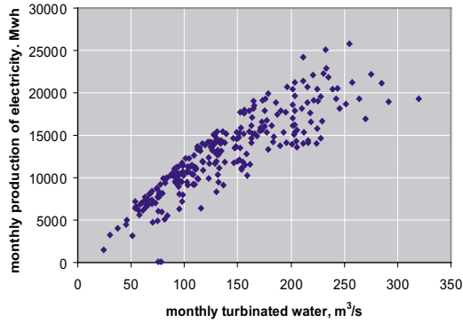
Fig. II.2. Sélingué: average turbine flow versus monthly generated energy
