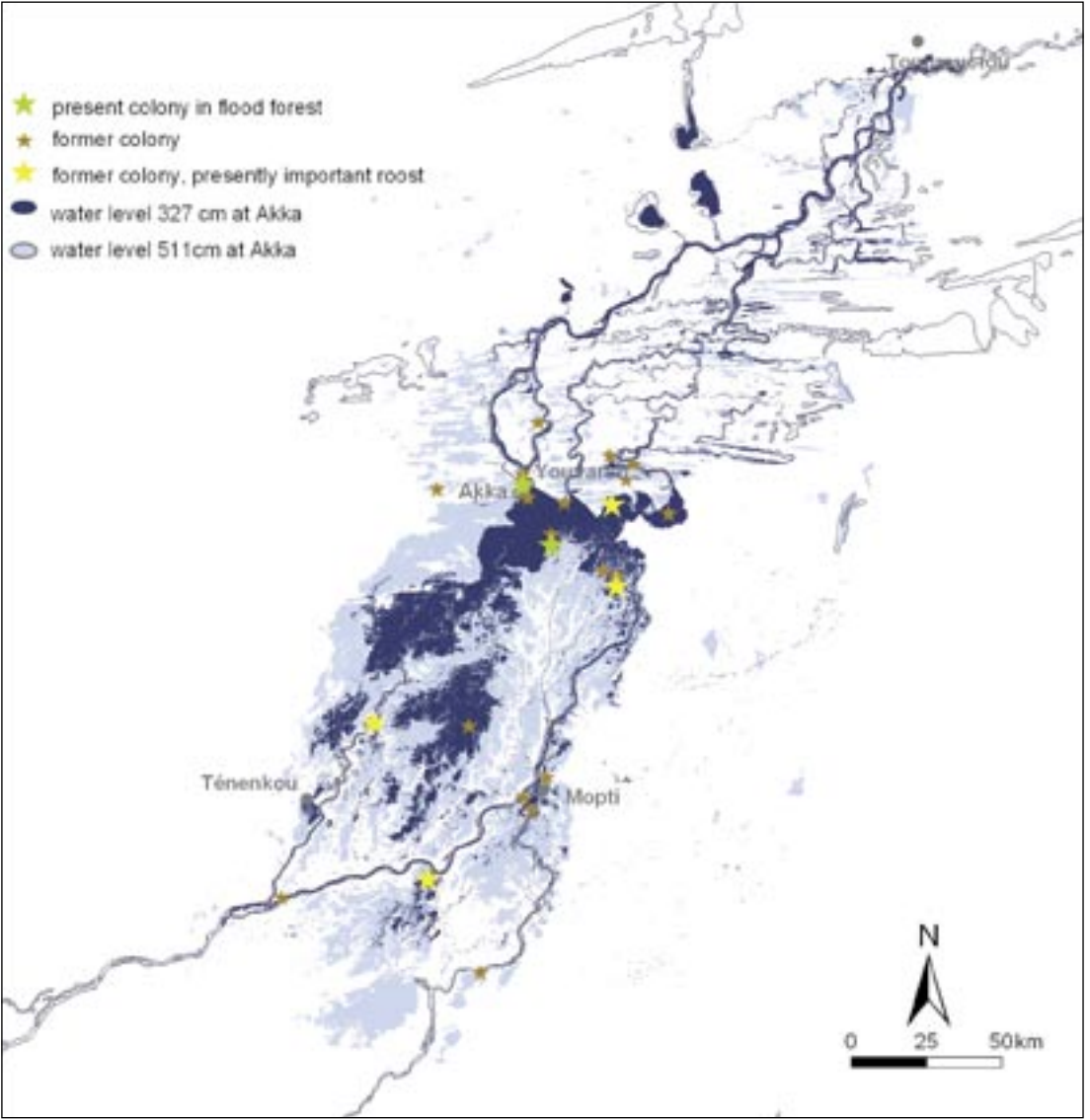
Fig. 9.3. Location of flood forests and breeding colonies in the Inner Delta in 2000-2004. At present two large breeding colonies exist in the (protected) flood forests of Akkagoun and Dentaka, whilst the other (fragments) of flood forests (resp. Pora, Niasso, Gourao, Bouna) are important roost sites for cormorants, herons and ibises (non-breeding adults, juveniles). Also former colony sites are shown (after Skinner et al. 1987).
